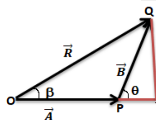
Fig. 2.11 Vector addition by Triangle law
