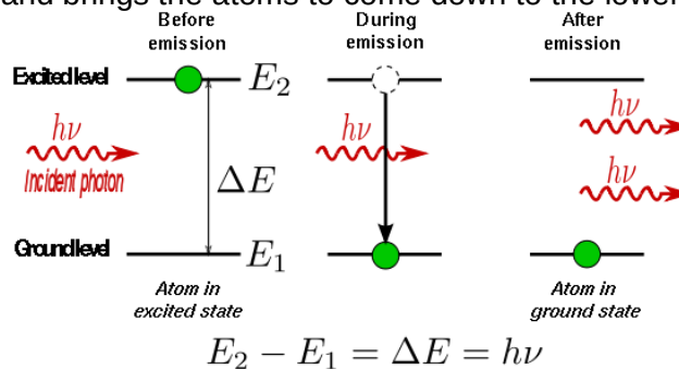
Stimulated emission (Fig. 12.3)
