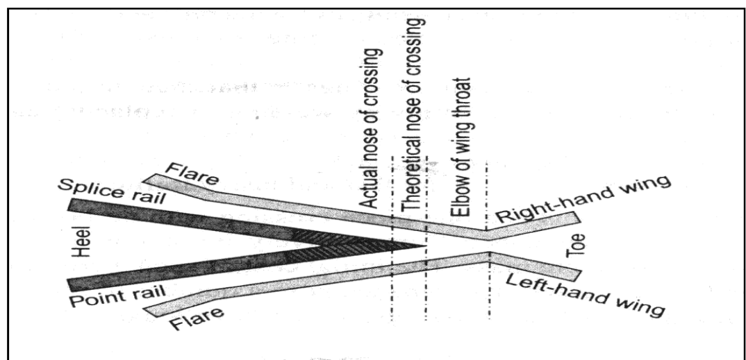
Figure:-PointRailandSpliceRail
