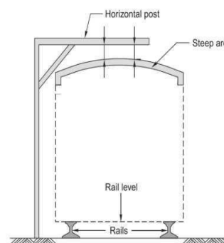
Fig. 2.2 Loading gauge
