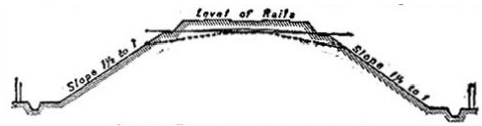
Typical Section of Railway in embankment.
