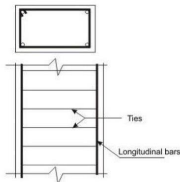
Tied Column
