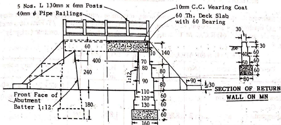
HALF CROSS SECTIONAL ELEVATION AT ABCD
