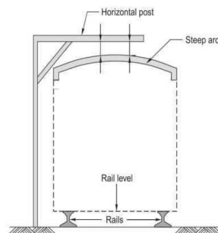
Fig. 2.2 Loading gauge
